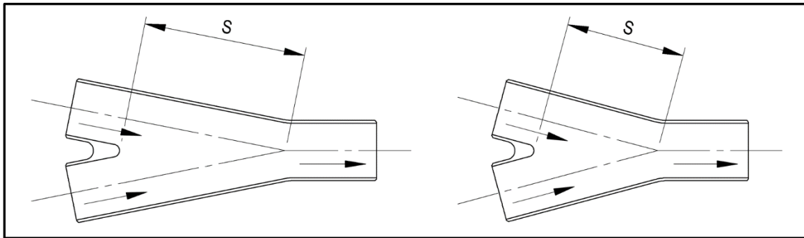
Figure 9 - Typical Piggable Wye Fittings
